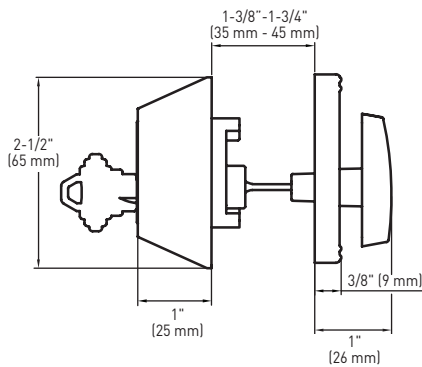
A. SINGLE CYLINDER DEADBOLT
