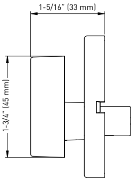
PRO SQUARE DEADBOLT INSIDE TRIM KIT
